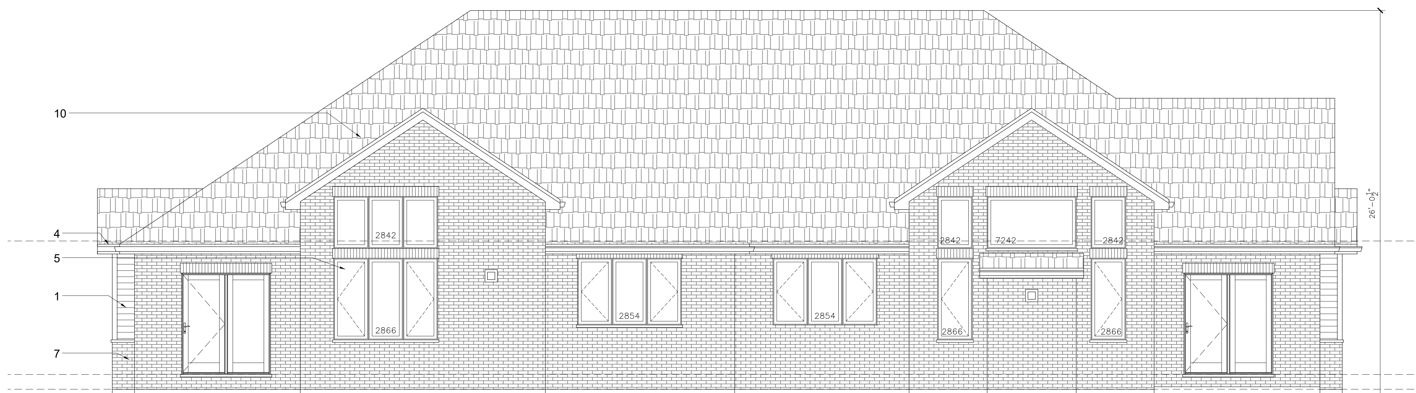
REAR ELEVATION 1/4" = 1'-0"
